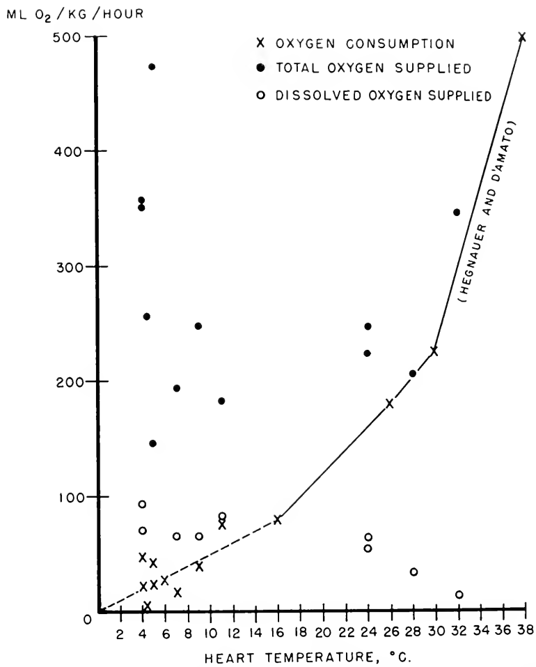
FIG. 5.—Oxygen consumption and oxygen supply in severe hypothermia with pump-oxygenator.
